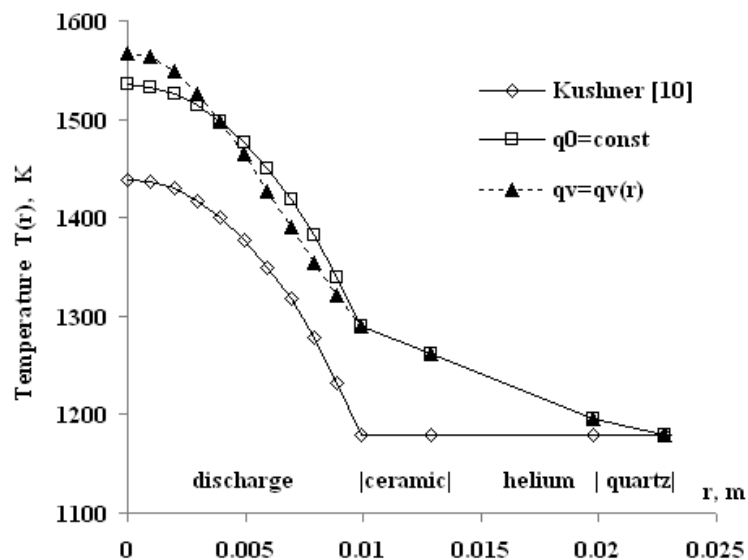
Figure 2. Distribution of the radial temperature profile in a half cross-section of the laser tube, found by the tree different models at total input electric power
