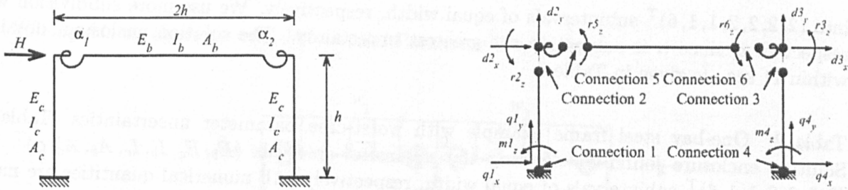
Figure 1: One-bay structural steel frame [5].
