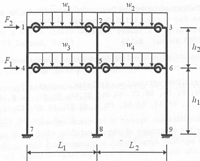
Figure 2: Two-bay two-story steel frame [29].
